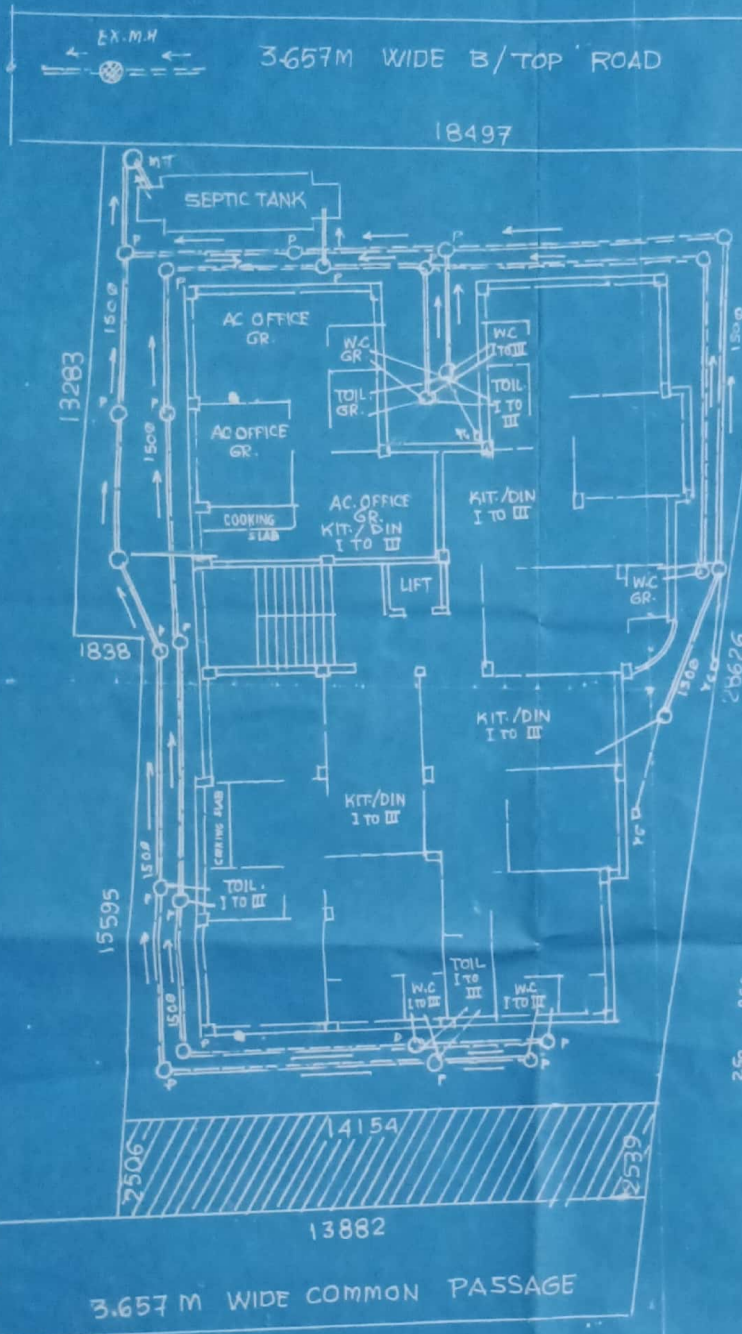
DETAILS OF SEPTIC TANK
